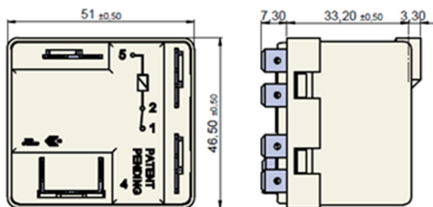
PANEL MOUNT (Quick-connect Terminal)
