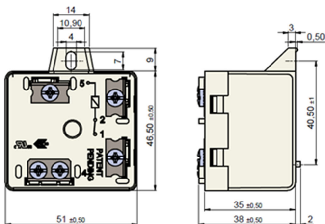
TAB MOUNT (Screw Terminal)
