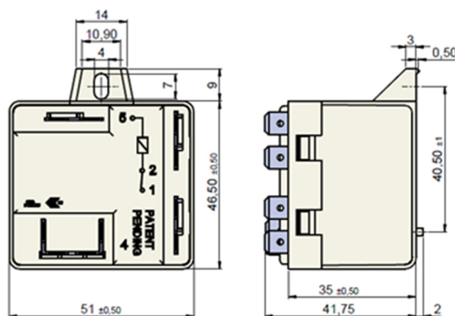
TAB MOUNT (Quick-connect Terminal)
